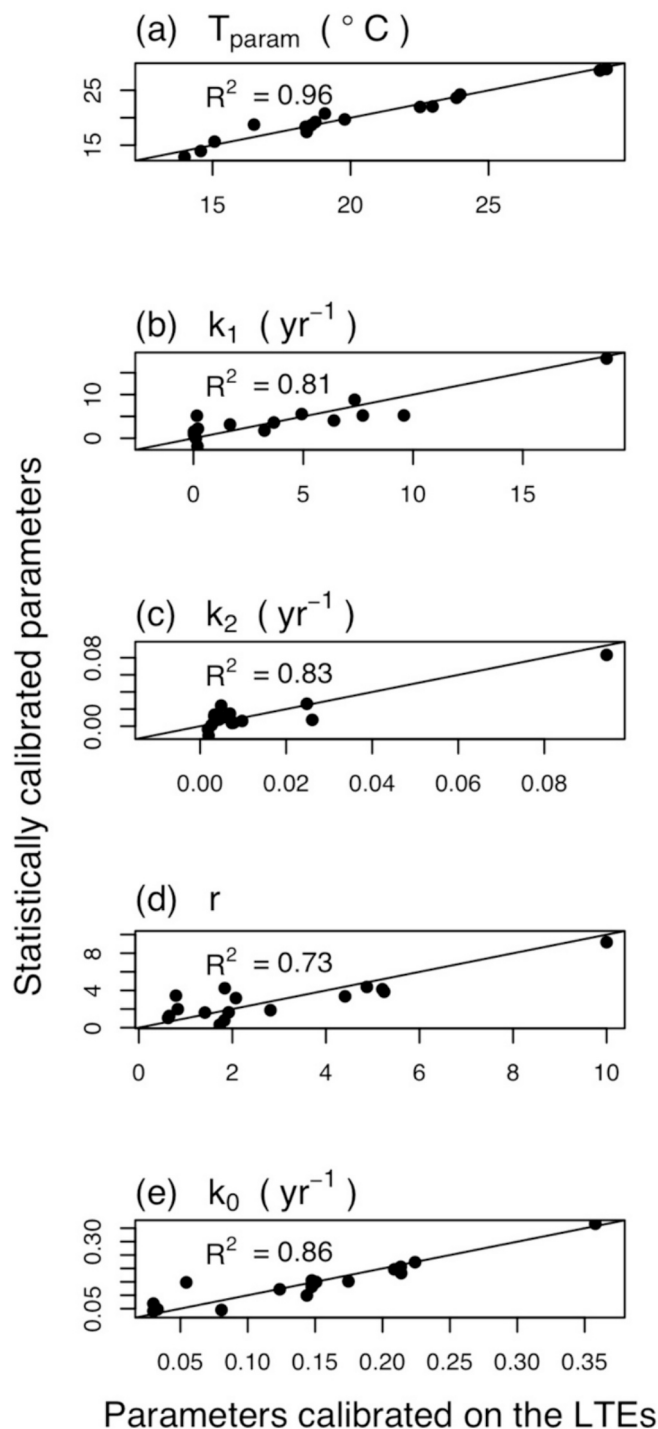
Fig. 2. Correlation between the predicted SOC model parameters estimated with the multiple linear regression (see Table 1), and the calibrated parameters estimated by fitting the SOC models to the measured SOC stock evolution in the 16 LTEs. (a) T_{\text{param}} ( ^{\circ}\text{C} ) is the reference temperature parameter of the temperature control function in the Roth-C model, (b) k_1 ( \text{yr}^{-1} ) and (c) k_2 ( \text{yr}^{-1} ) are the decomposition rate parameters of the young and the old pool in the ICBM model, respectively, (d) r is the environmental modifier in the ICBM model, and (e) k_0 ( \text{yr}^{-1} ) is the decomposition rate parameter of the active pool in the AMG model.
