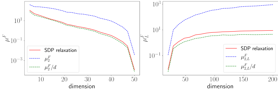
Figure 8: Comparison of the SDP relaxation for \mu_1^F on the left (resp. \mu_{1,L}^F on the right) with \mu_2^F and \mu_2^F/d (resp. \mu_{2,L}^F and \mu_{2,L}^F/d ) for a random feature model generated from the Leukemia dataset with a number of samples n = 50 (resp. n = 20 ).
