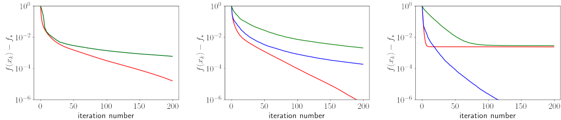
Figure 3: Convergence in function value of the proximal gradient descent, coordinate descent with Gauss-Soutwhell rule and with L = L_1^F (instead of L = L_2^F ) and of the regularized matching pursuit, for synthetic quadratics (see Section 2.3) with n = 50 , s = 8 , \lambda = 0.001 , \sigma = 0.5 and for d = 30 starting from zero on the left (underparametrized regime), from a non zero point in the middle (underparametrized regime) and for d = 500 on the right (overparametrized regime). RMP and coordinate descent with GS-rule match exactly in these examples.
