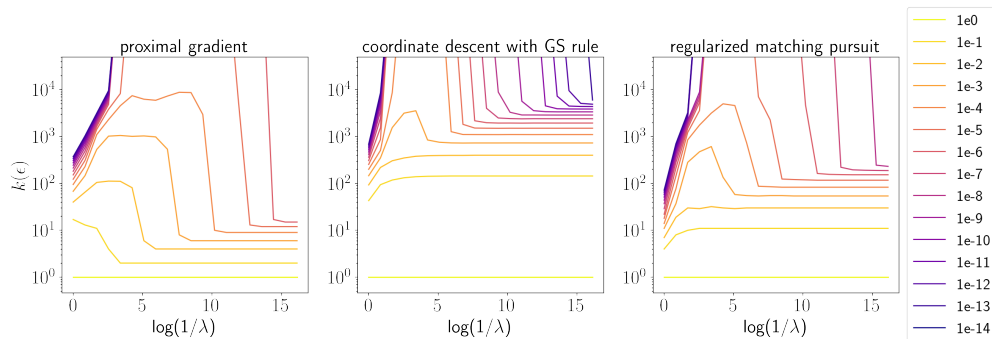
Figure 5: \epsilon -curve of the proximal gradient, coordinate descent with the GS rule and regularized matching pursuit for a LASSO problem with d = 500 , n = 50 , a sparsity level s = 8 , \sigma = 0.5 , after k = 10000 iterations for several values of \lambda .
