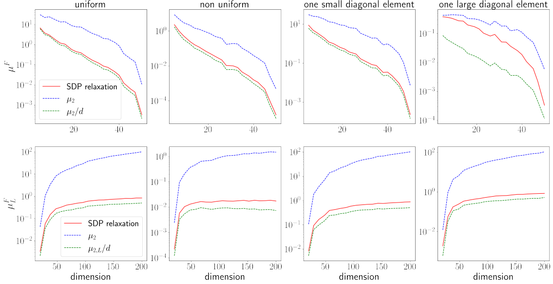
Figure 7: Comparison of \mu_1^F on the top (resp. \mu_{1,L}^F on the bottom) with \mu_2^F and \mu_2^F/d (resp. \mu_{2,L}^F and \mu_{2,L}^F/d ) for n = 50 (resp. n = 20 ) averaged on 5 trials, for Gaussian random data with a variance equal from the left to the right to \Sigma = I_d , \Sigma = \text{diag}(1, 1/2, \dots, 1/d) , \Sigma = \text{diag}(1, \dots, 1, 1/100) and \text{diag}(1, \dots, 1, 100) .
