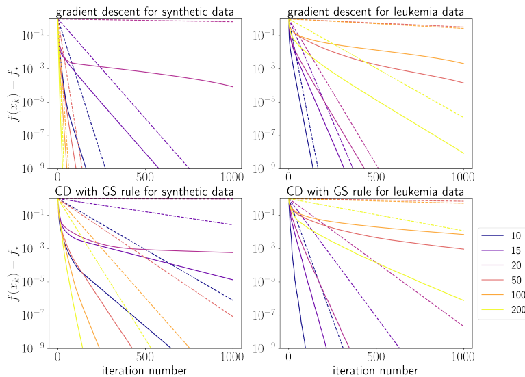
Figure 2: Convergence in function value for gradient descent and coordinate descent with GS rule, on synthetic quadratics ( n = 20 ) and on the leukemia dataset ( n = 72 ), for different values for d . Dashed lines: comparison to the approximate convergence guarantees from Corllary 6 for synthetic quadratics, and to high probability estimates for the leukemia dataset from Proposition 9.
