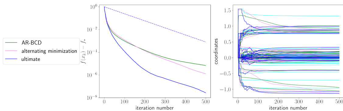
Figure 9: Convergence in function value for the ultimate method computed with an alternating minimization technique, AR-BCD, and with the solver MOSEK, compared to the regularized matching pursuit. Parameters are given by d = 50 , n = 20 , s = 8 and \lambda = 0.001 , with an inner loop with exponential precision.
