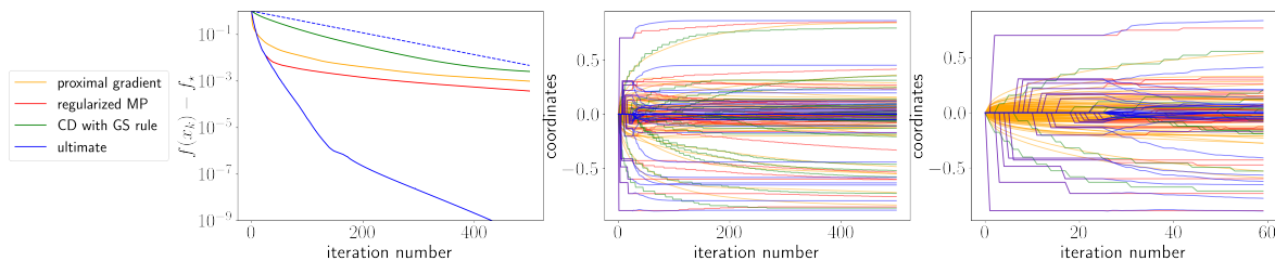
Figure 6: Convergence in function value and coordinates as a function of the iteration number for the proximal gradient descent, the proximal coordinate descent with GS rule, the regularized matching pursuit and the ultimate method on a LASSO problem, with d = 500 , n = 50 , s = 8 , \lambda = 0.2 . The approximate guarantee in provided in dashed lines.
