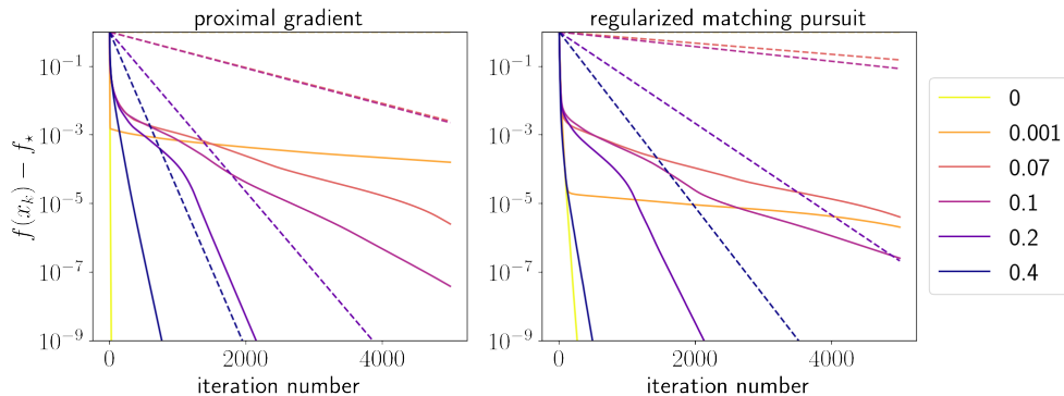
Figure 4: Convergence in function values for the proximal gradient on the left and the regularized matching pursuit on the right for n = 50 , d = 500 and a sparsity s = 8 and for several penalty \lambda . Convergence is compared in dashed lines to local convergence guarantee, taken on the support S on the last iterates and the SDP relaxation from Proposition 8.
