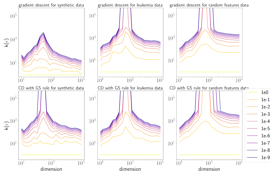
Figure 1: \epsilon -curve for gradient descent (top) and coordinate descent with the GS-rule (bottom), for the three models: synthetic quadratics (on the left) with n = 50 , the leukemia dataset (in the middle) with n = 72 , a random feature model (on the right) with n = 72 .
