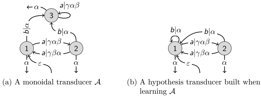
Figure 1: Two transducers: unlike automata, the transitions are also labelled with output words.
