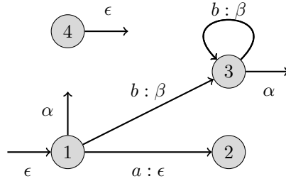
Figure 2: A monoidal transducer \mathcal{A}
