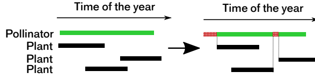
Figure 3: Phenological change in possible interaction between a pollinator and plants due to climate, after Memmott et al. (2007). Left: original situation. Right: situation after the change. For pollinators, the period represented is the period of activity, for the plants it is the period of flowering. In the case represented, every plant is pollinated; however, the pollinator has two periods without plants to pollinate after the change.
