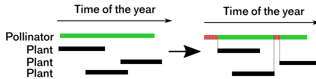
Figure 3: Phenological change in possible interaction between a pollinator and plants due to climate, after Memmott et al. (2007) . Left: original situation. Right: the situation after the change. For pollinators, the period represented is the period of activity; for the plants, it is the period of flowering. In the case represented, every plant is pollinated; however, the pollinator has two periods without plants to pollinate after the change.
