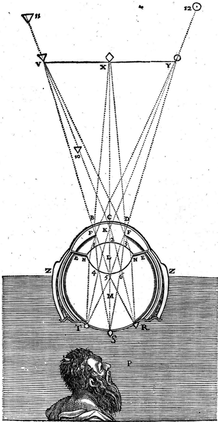
Figure 12: Graphical conventions of Descartes' Dioptrique , in Descartes, 1964–1974, vol. VI, 106.
