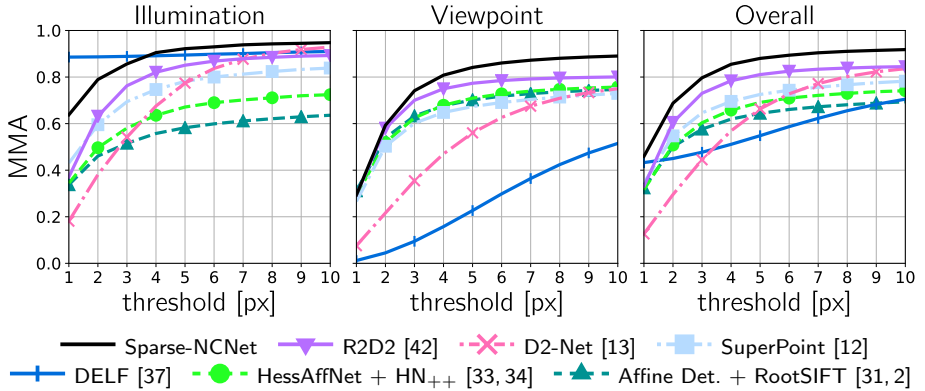
Fig. 5: Sparse-NCNet vs. state-of-the-art on HPatch. The MMA of Sparse-NCNet and several state-of-the-art methods is shown. Sparse-NCNet obtains the best results overall with a large margin over the recent R2D2 method.
