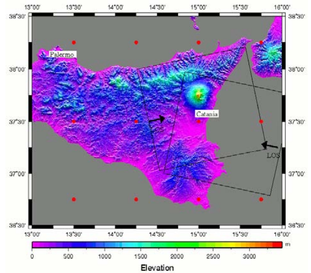
Figure 2. Topographic map of Sicily. Boxes indicate coverage of Envisat scenes on ascending and descending tracks. Only data from ascending (east looking) track are used in this study. Dots indicate location of ERAI grid nodes.
