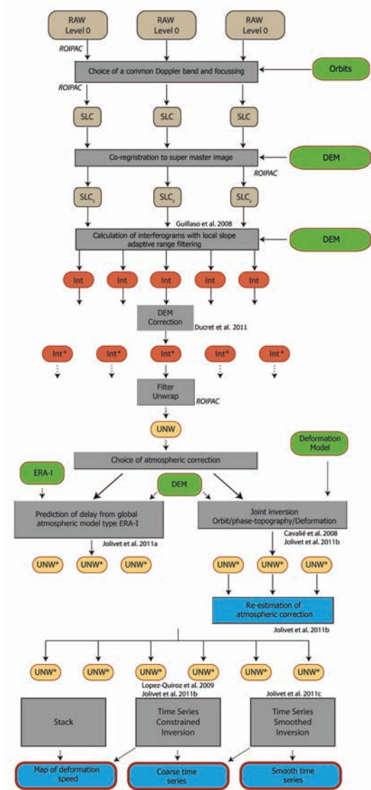
Figure 1. Diagram showing the NSBAS chain steps (Romain Jolivet, thesis)
