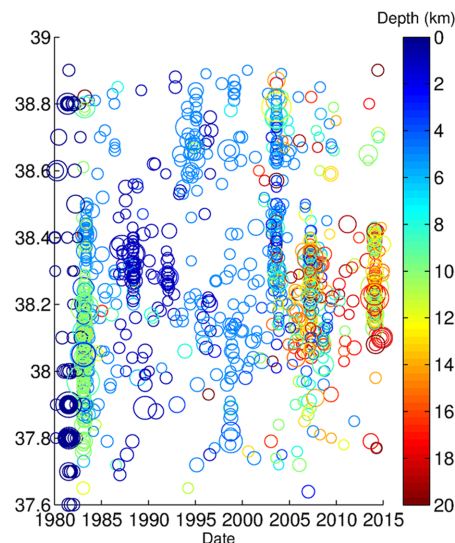
Figure 18. Spatio-temporal evolution of the seismicity (from the NOA catalogue) from 1980 to 2015 along the CTF, plotted with latitude function of date. The events are those located between the two hatched white lines of Fig. 17, with magnitude larger than 3.5 and shallower than 20 km. The clustering in time and space of the seismicity is clear, as well as the gap of seismicity between Cephalonia and Lefkada. The 2003 sequence has two patches. The northern one is well correlated with the observed ground deformations (from GPS and SAR interferometry). The southern one, with little or no related deformation, is less understood.
