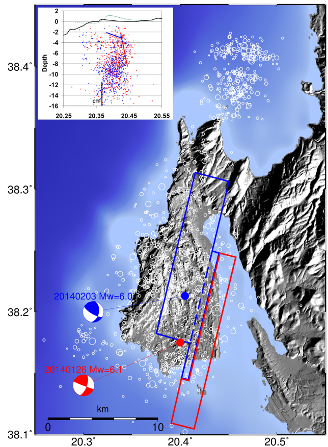
Figure 16. Projection of the faults inferred for the January 26 earthquake (red) and the February 3 earthquake (blue) with the seismicity relocated between January 26 and February 18 by Karakostas et al. (2015) and the C-GMT focal mechanisms. The fault of the February 3 event has two elements, one coplanar with the January 26 fault and the other one with low angle. The direction of slip is shown with the thick arrows. The figure in inset shows a cross section along a N102^\circ direction (A–A' section) with in red and blue the location of the faults, in hatched black the location of the CTF as inferred from the interseismic GPS data, in solid black the topography, and in dotted green the vertical displacement that would be produced by 10^4 events similar to the one we have estimated for the 2014 sequence. Most of the aftershock sequence occurs in the longitude domain located between the CTF and the 2014 faults.
