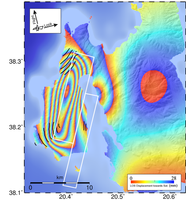
Figure 13. Best-fitting model for the entire sequence. Observed (picked fringes in black) and modelled RS2 interferogram. The rectangles show the projection of the modelled fault, both dipping east, the main strike-slip fault is located deeper and south and the one located to the north is shallower with a lower dip angle. The average scatter between RS2 observation and model is 26 mm.
