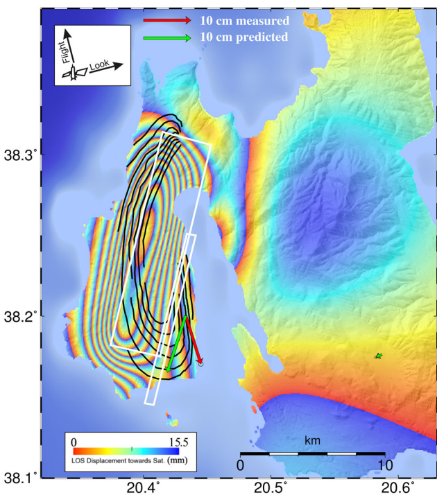
Figure 14. Best-fitting model for the February 3 earthquake. Observed (picked fringes in black) and modelled TSX interferogram. Observed and modelled displacements at KEFA and VLSM GPS stations. The rectangles show the location of the two elements of the modelled fault. The average scatter between observation and model is 26 mm.
