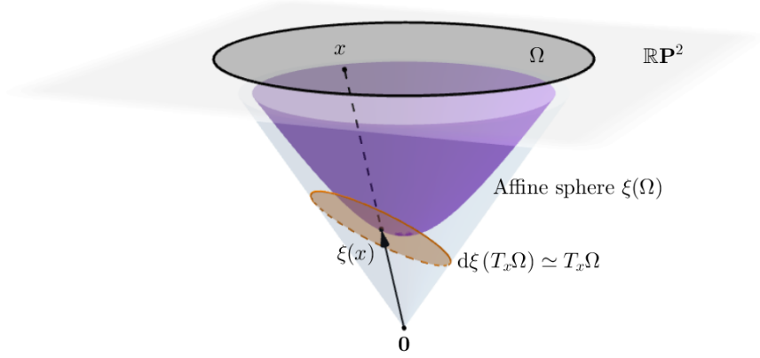
FIGURE 1. When \Omega is a disc in \mathbb{RP}^2 , the hyperbolic affine sphere asymptotic to \Omega is a hyperboloid.
